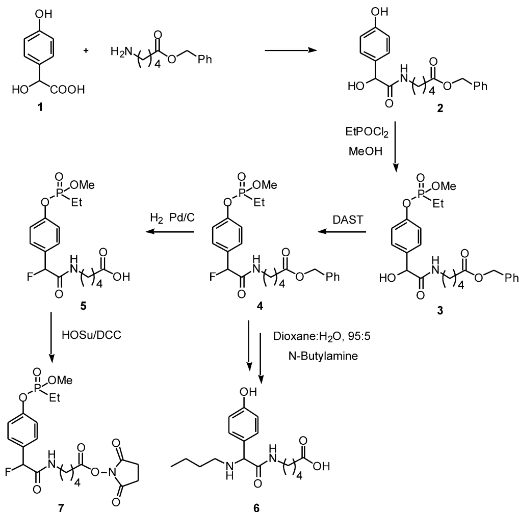
Scheme 2. Synthesis of hapten 7.
