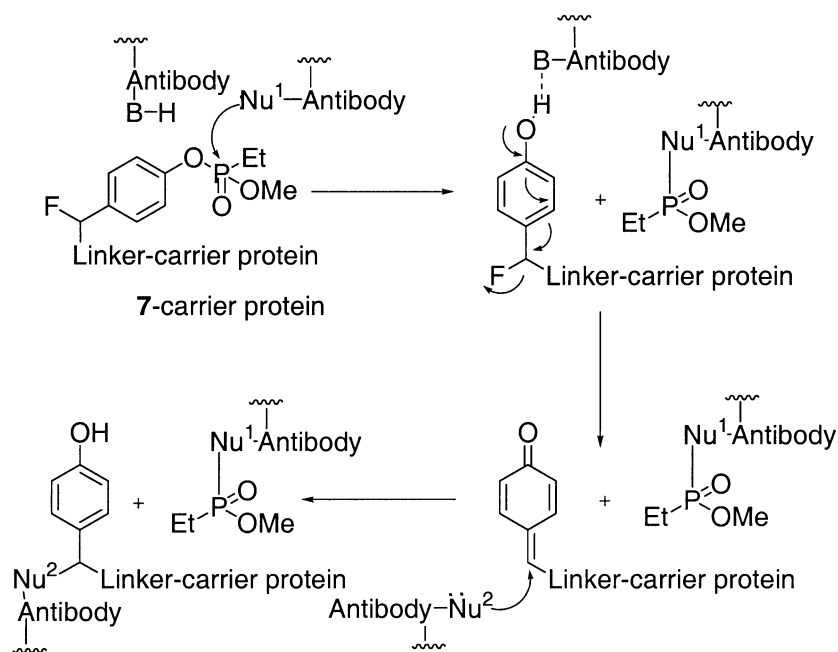
Scheme 3. Double reactive immunization with hapten 7.
