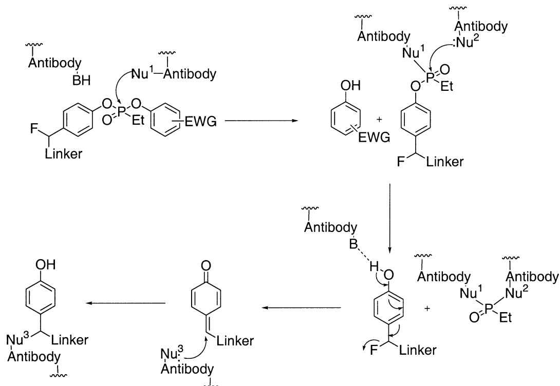
Scheme 4. Multiple reactive immunization leading to three different nucleophile catalytic residues in the antibody binding site.
