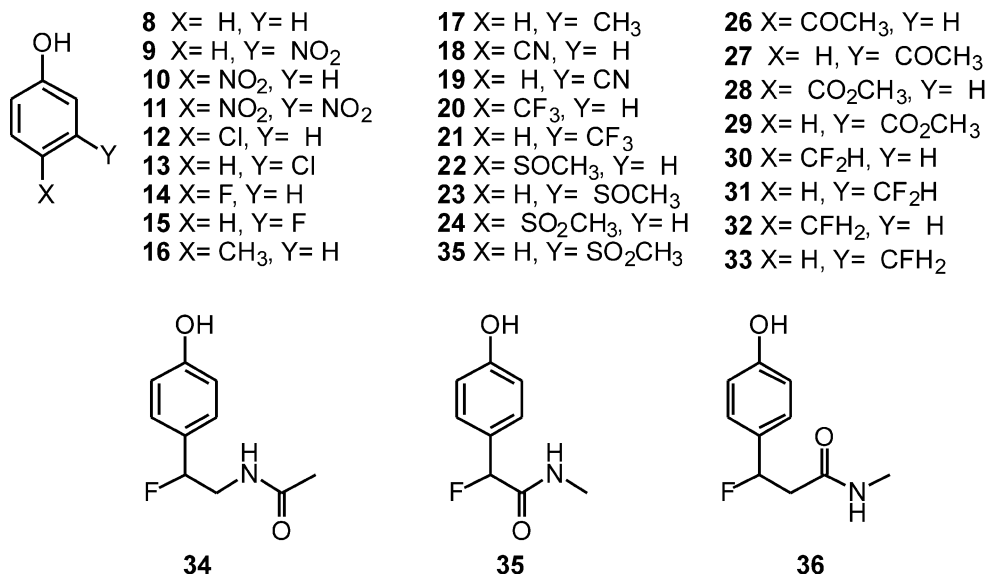
Figure 1. Structures of phenols used for pK a calculations.
