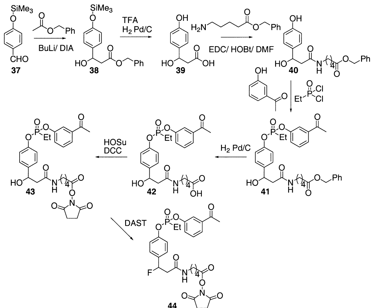
Scheme 5. Synthesis of hapten 44.
