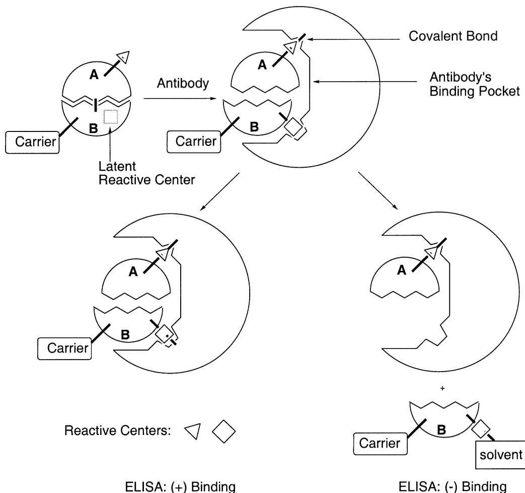
Scheme 1. Schematic representation of the multiple reactive immunization concept.
